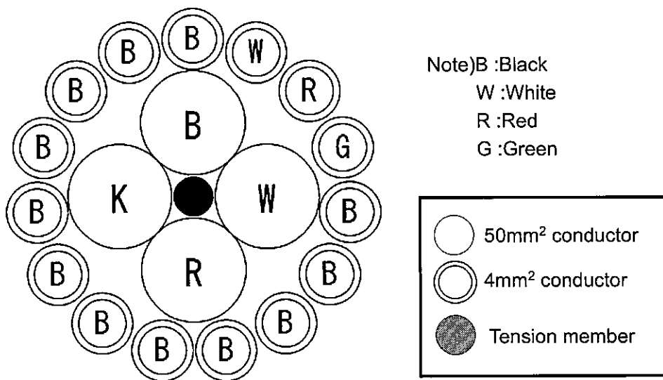
Fig.2. Core identification
